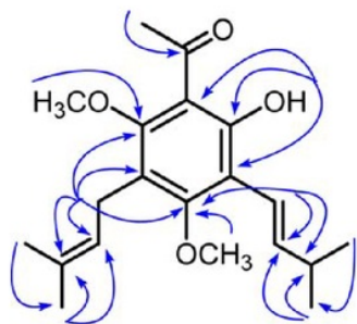
Fig. 2. Selected HMBC correlations for compound 1 .
